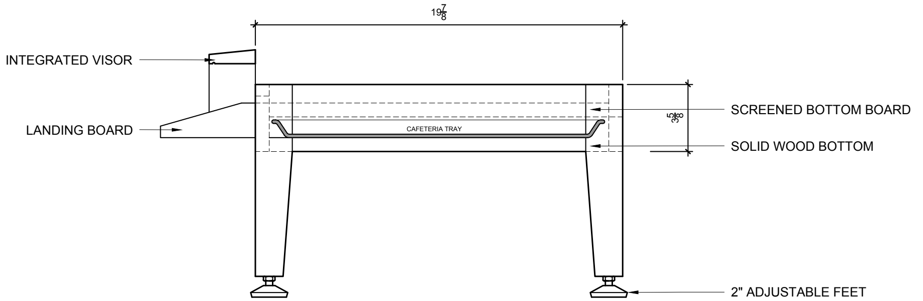
LANGSTROTH BASE SECTION w/ INTEGRATED IPM
