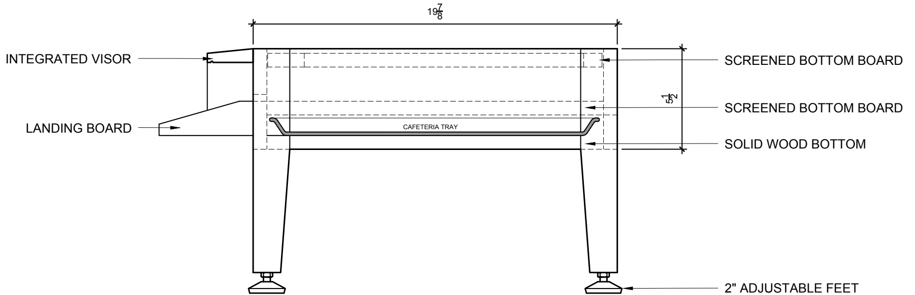
LANGSTROTH BASE SECTION w/ INTEGRATED IPM & SLATTED RACK
